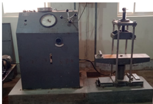
Flexural testing machine set up
